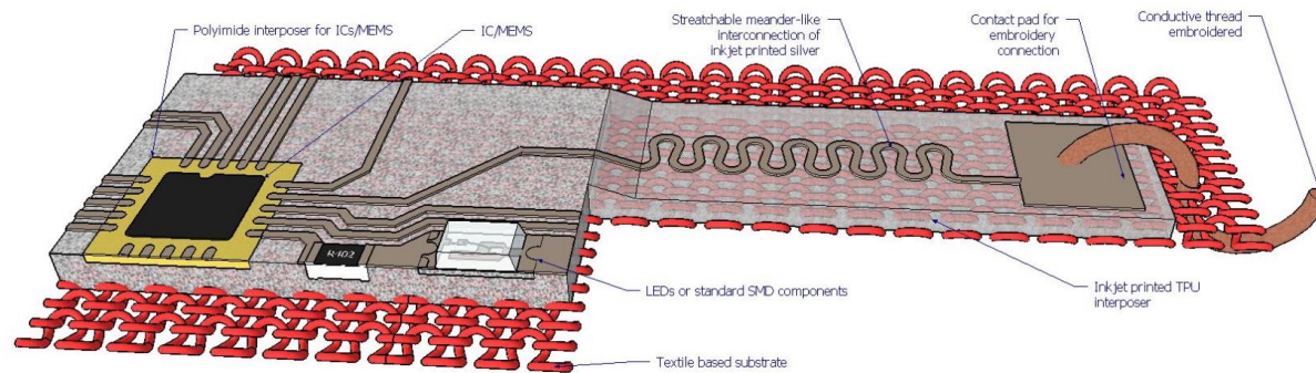
Printed interposer
